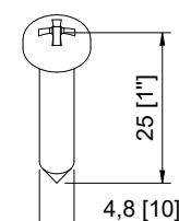
290171 PARAFUSO CQ 1x10 INOX
