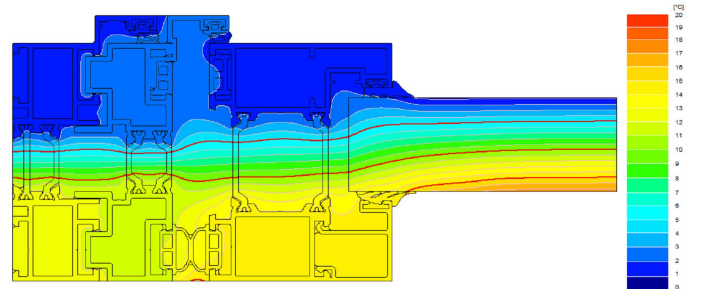
Secção | Section | Section (10b) U_f = 3,11 \text{ W/m}^2\text{K}
