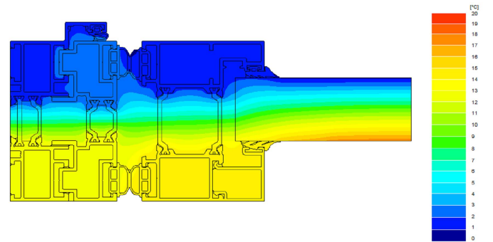
Secção | Section | Section (2b) U_f = 3,05 \text{ W/m}^2\text{K}
