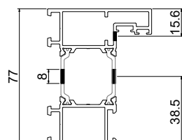
Corte | Cut | Coupe K-K
