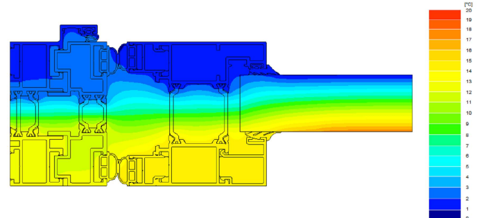
Secção | Section | Section (6b) U_f = 3,08 \text{ W/m}^2\text{K}
